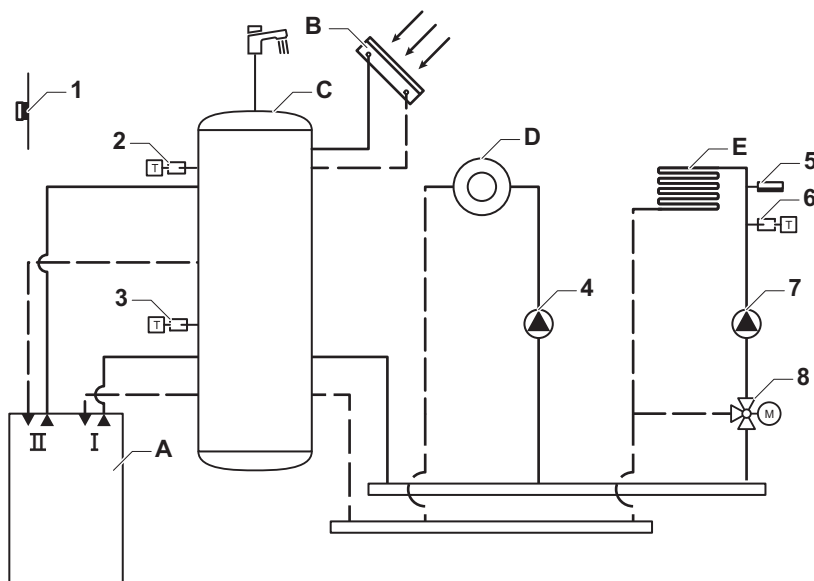
Afb.56 1 ketel + 1 combi-bufferboiler + 1 directe zone + 1 mengzone + zonnecollectoren
