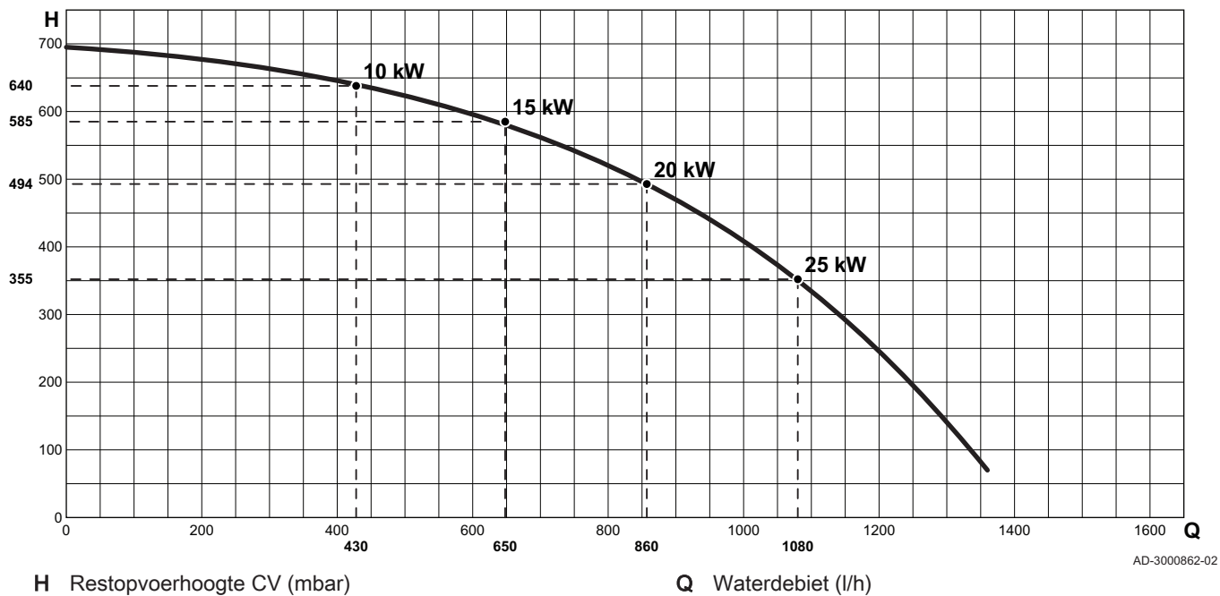
Afb.3 AMC 24/28 BIC
