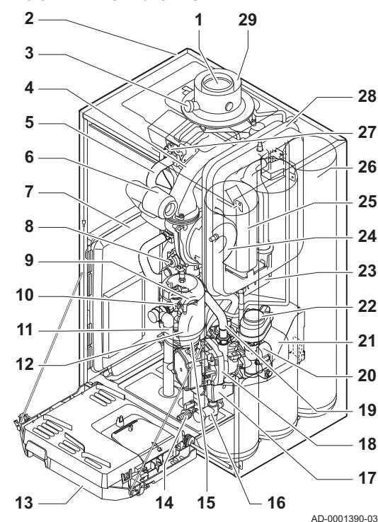
Afb.5 AMC 24/28 BIC
